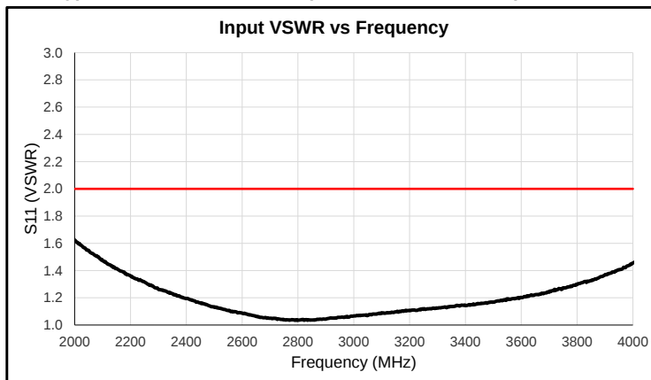
Typical Performance @ 23°C (Reference S/N 2151298)
